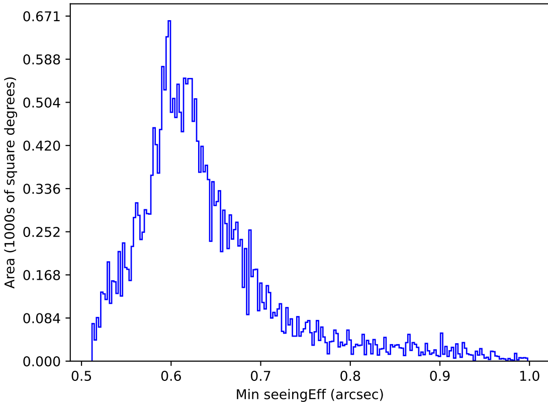
ddf_loaded_fl15_v3.4_10yrs All sky i band: Min seeingEff
