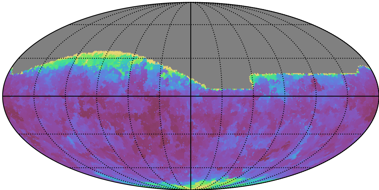
ddf_loaded_fl15_v3.4_10yrs All sky g band: Min seeingEff
