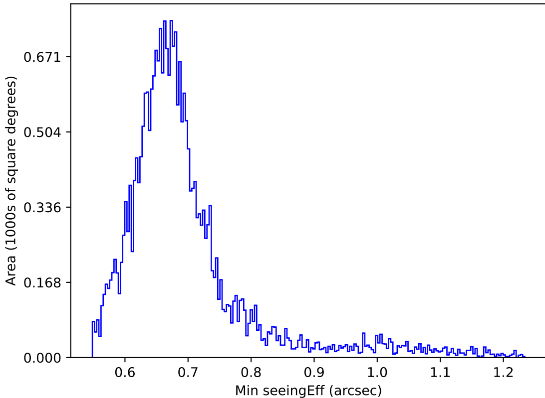
ddf_loaded_fl15_v3.4_10yrs All sky g band: Min seeingEff
