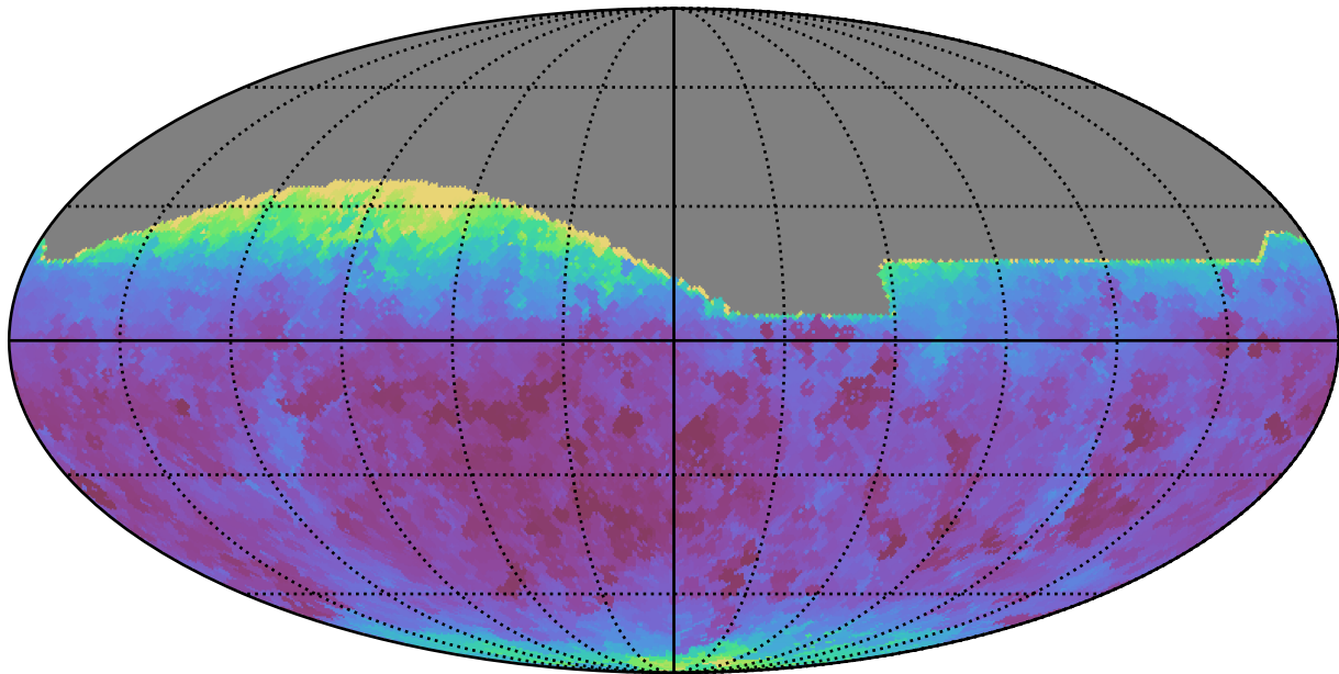
ddf_loaded_fl15_v3.4_10yrs All sky all bands: Min seeingEff
