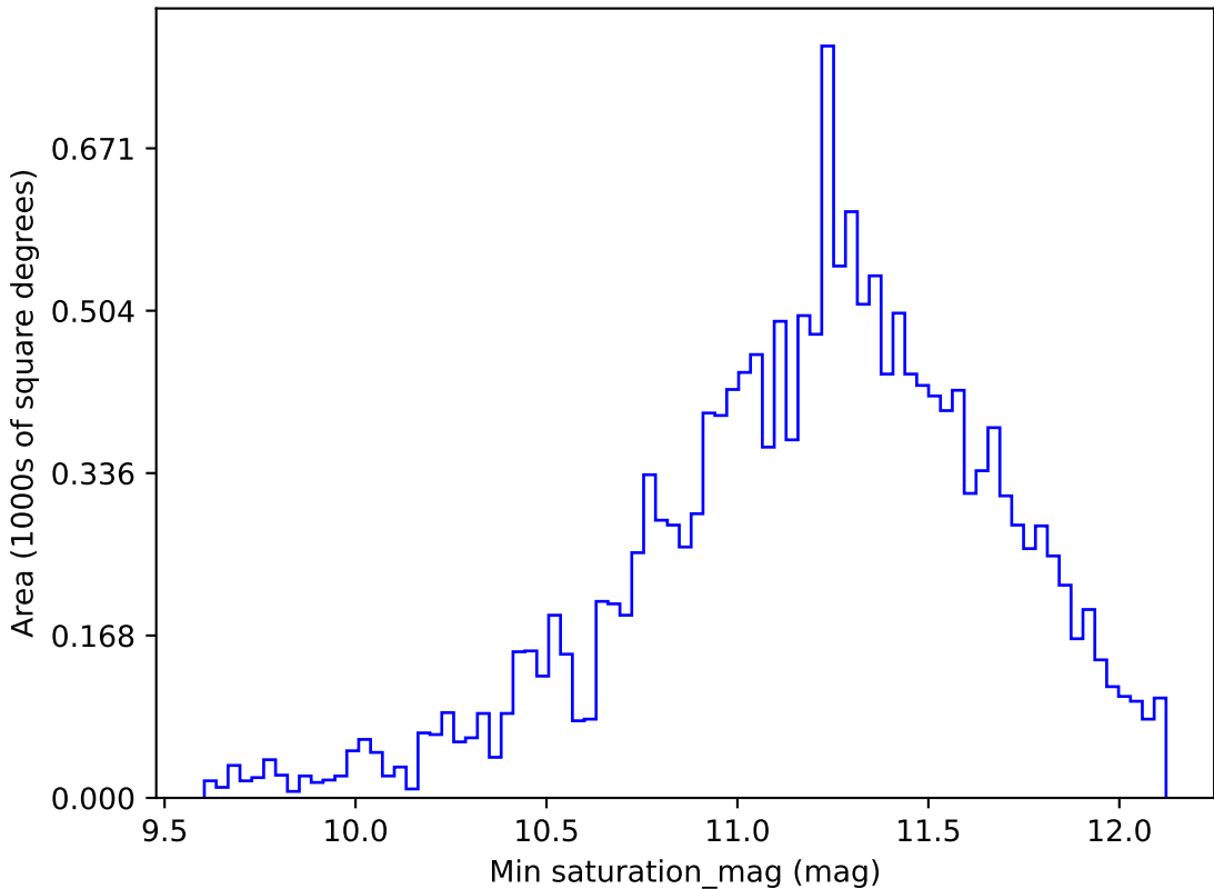
ddf_loaded_fl15_v3.4_10yrs WFD y band: Min saturation_mag
