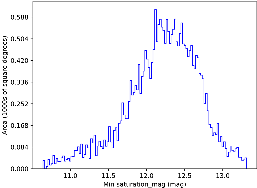
ddf_loaded_fl15_v3.4_10yrs All sky z band: Min saturation_mag
