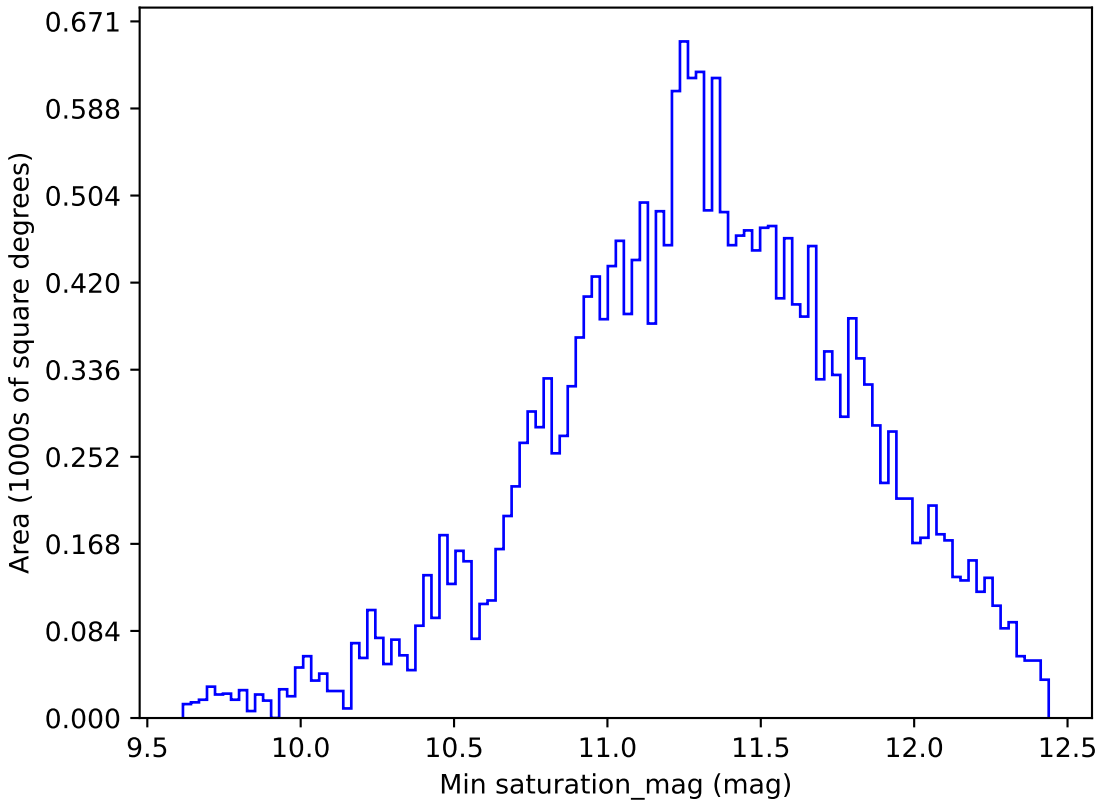
ddf_loaded_fl15_v3.4_10yrs All sky y band: Min saturation_mag
