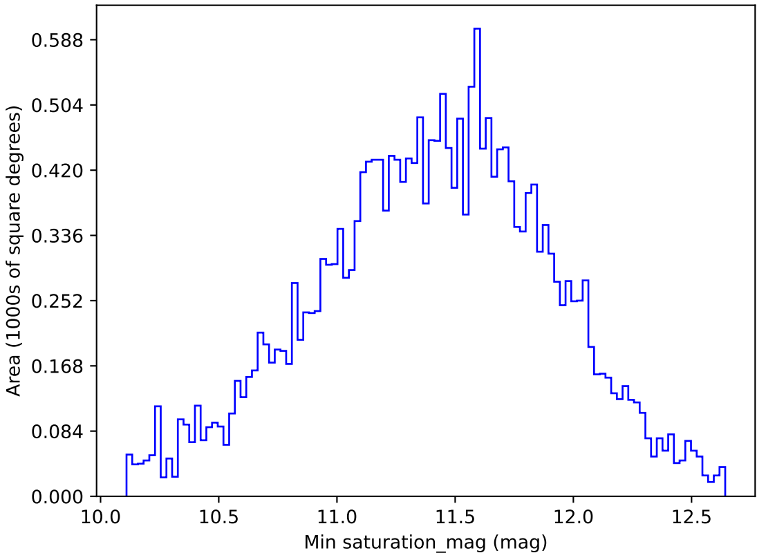
ddf_loaded_fl15_v3.4_10yrs All sky u band: Min saturation_mag
