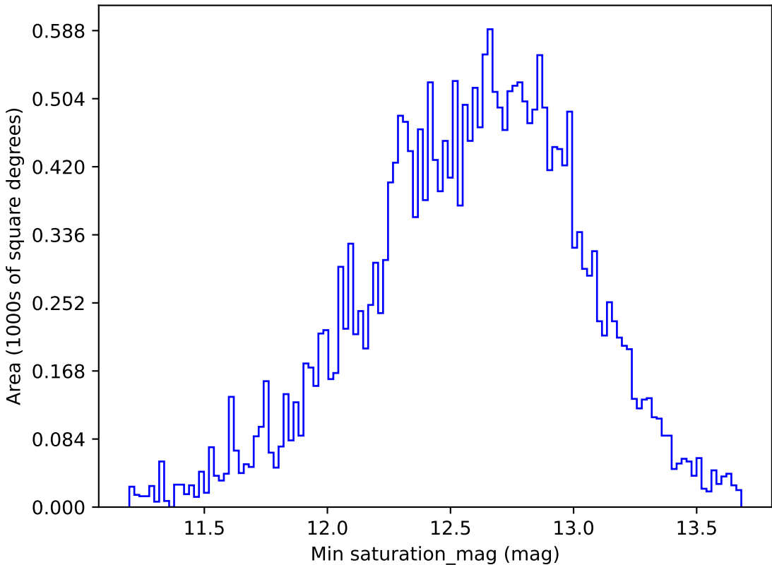
ddf_loaded_fl15_v3.4_10yrs All sky r band: Min saturation_mag
