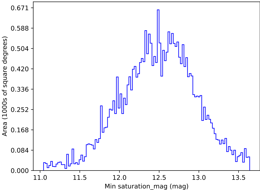
ddf_loaded_fl15_v3.4_10yrs All sky i band: Min saturation_mag
