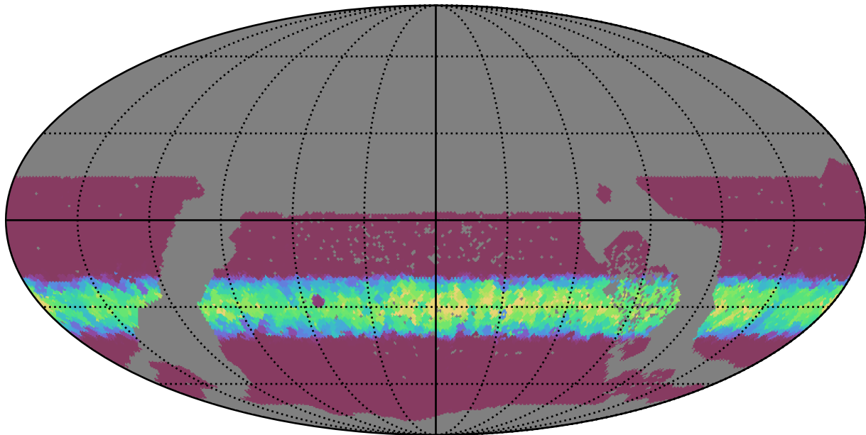
ddf_loaded_fl15_v3.4_10yrs WFD z band: Min normairmass
