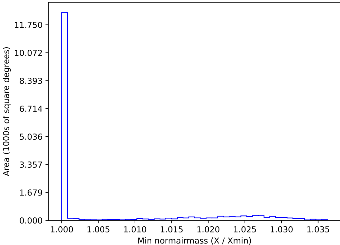
ddf_loaded_fl15_v3.4_10yrs WFD z band: Min normairmass
