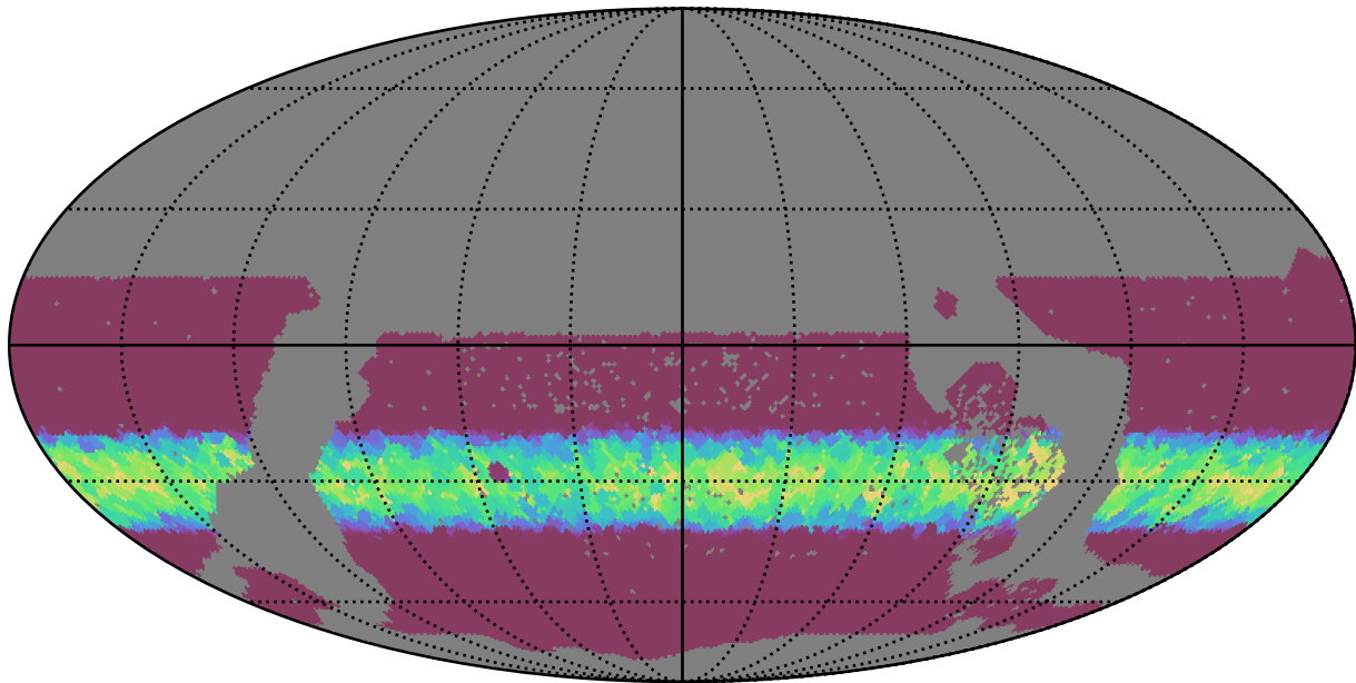
ddf_loaded_fl15_v3.4_10yrs WFD y band: Min normairmass
