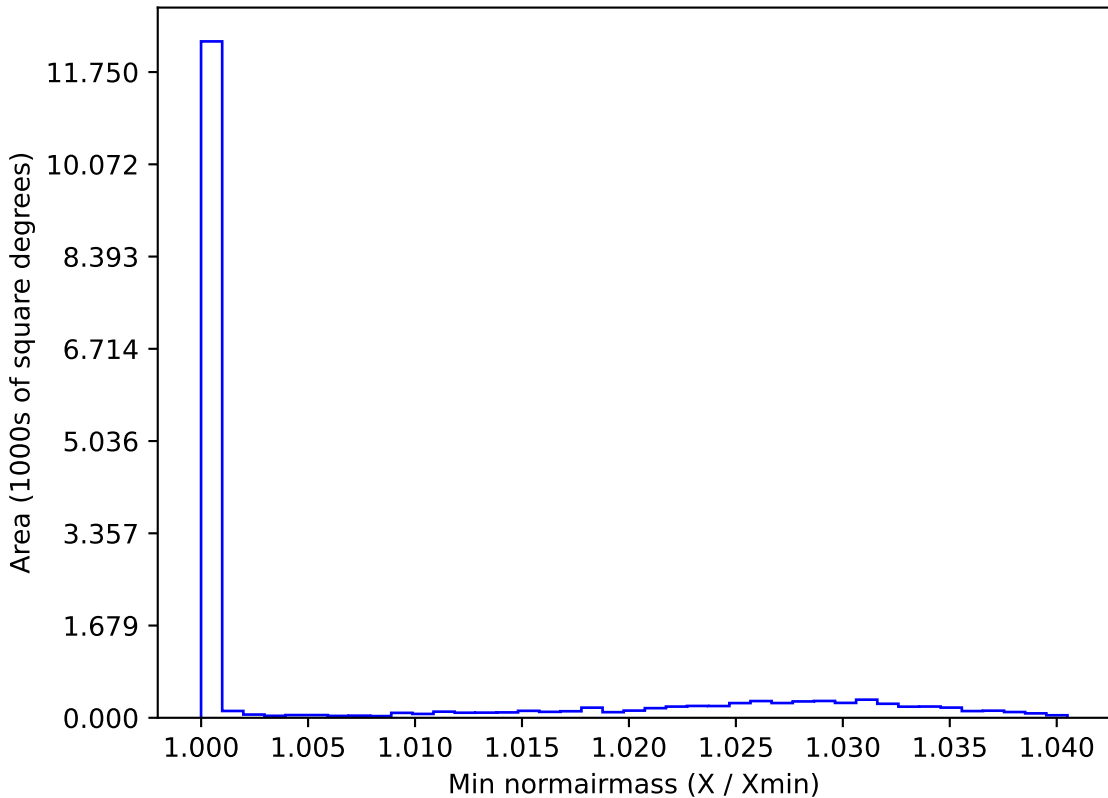
ddf_loaded_fl15_v3.4_10yrs WFD y band: Min normairmass
