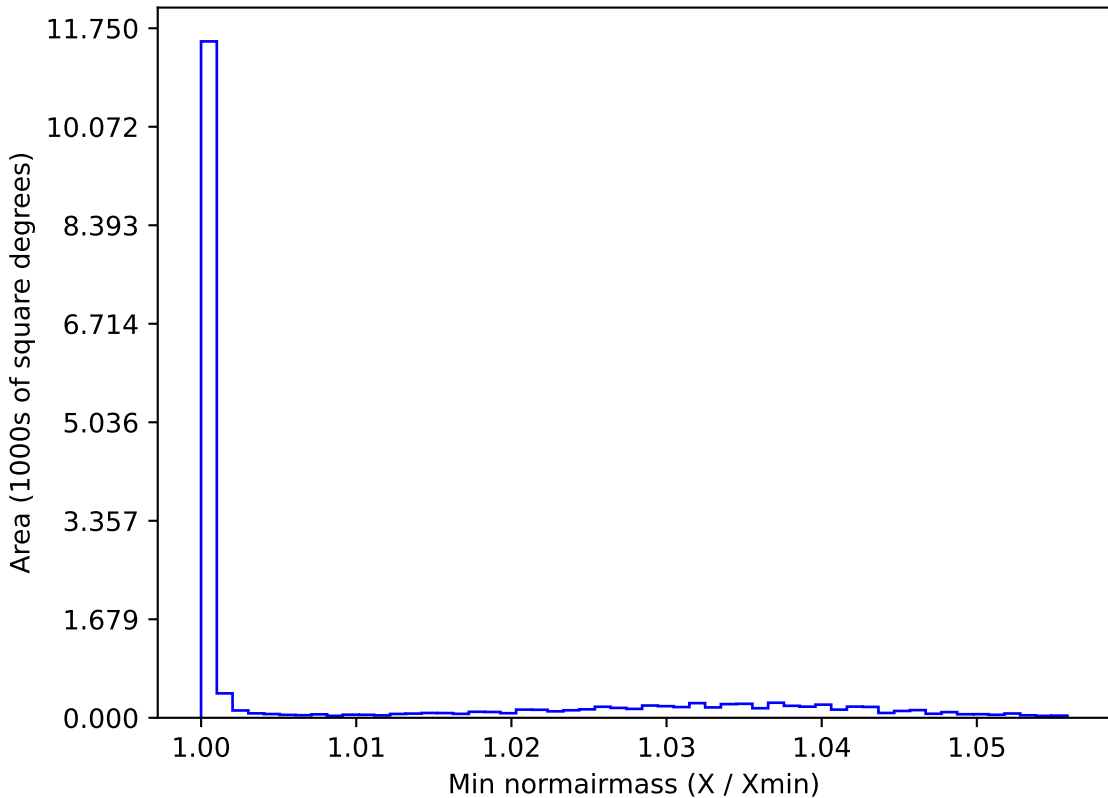
ddf_loaded_fl15_v3.4_10yrs WFD u band: Min normairmass
