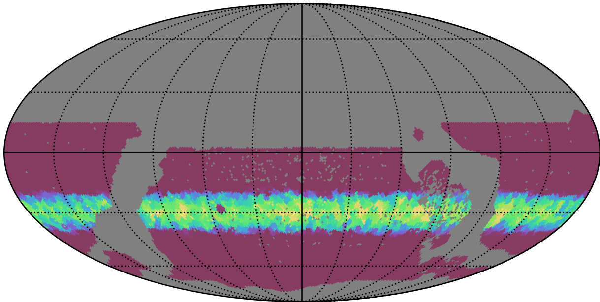
ddf_loaded_fl15_v3.4_10yrs WFD r band: Min normairmass
