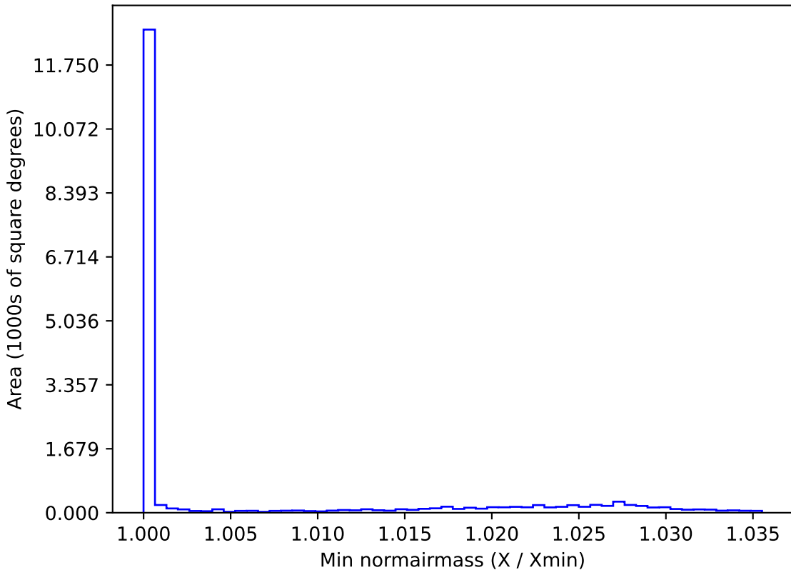
ddf_loaded_fl15_v3.4_10yrs WFD r band: Min normairmass
