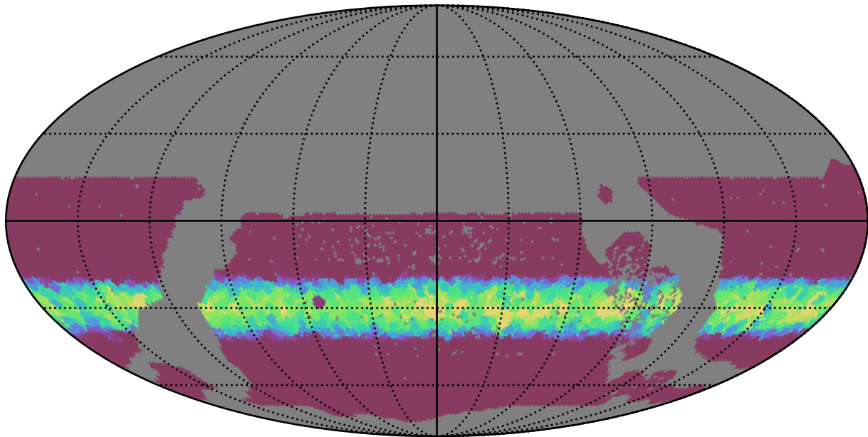
ddf_loaded_fl15_v3.4_10yrs WFD i band: Min normairmass
