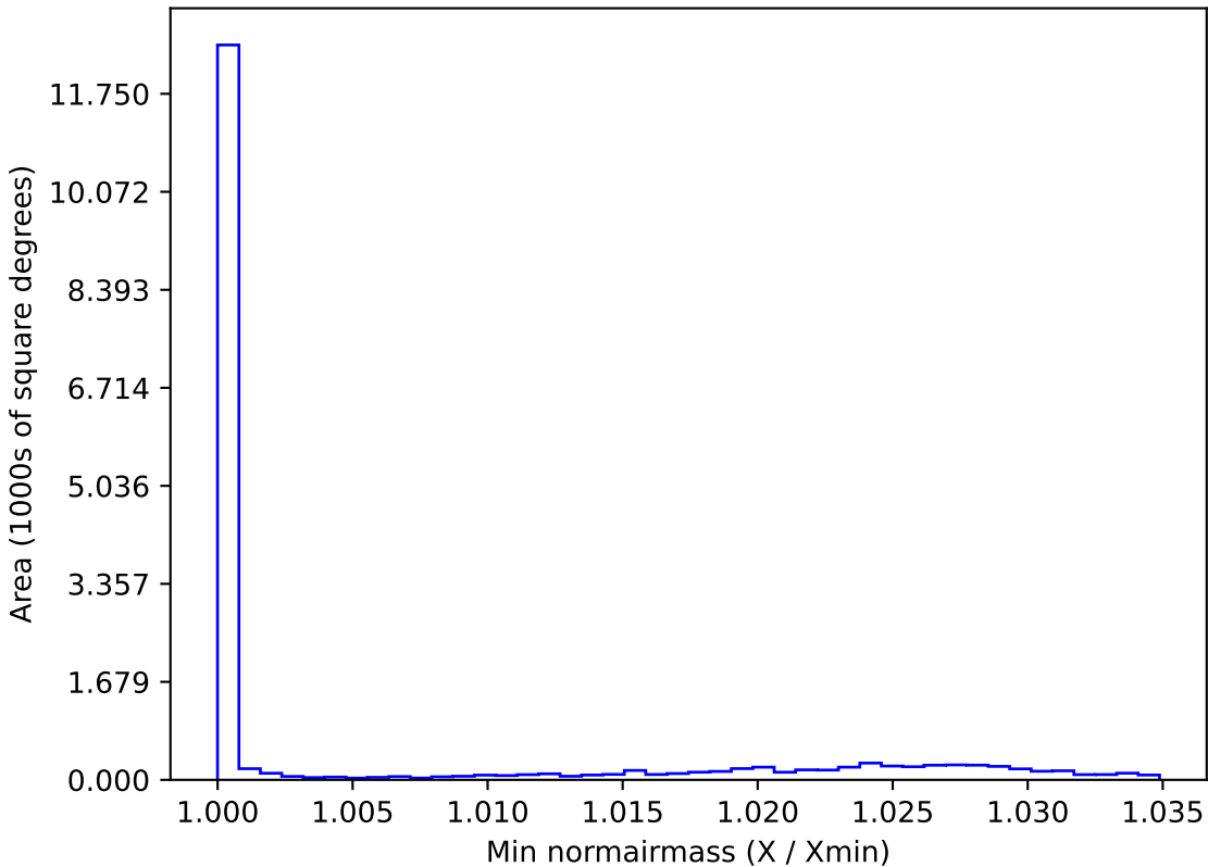
ddf_loaded_fl15_v3.4_10yrs WFD i band: Min normairmass
