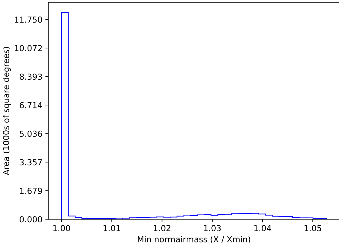
ddf_loaded_fl15_v3.4_10yrs WFD g band: Min normairmass
