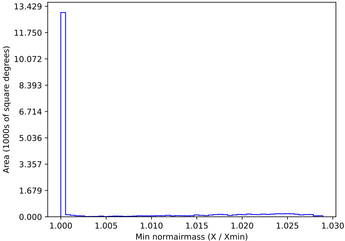
ddf_loaded_fl15_v3.4_10yrs WFD all bands: Min normairmass
