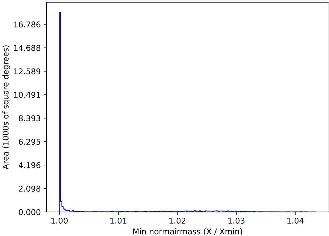
ddf_loaded_fl15_v3.4_10yrs All sky z band: Min normairmass
