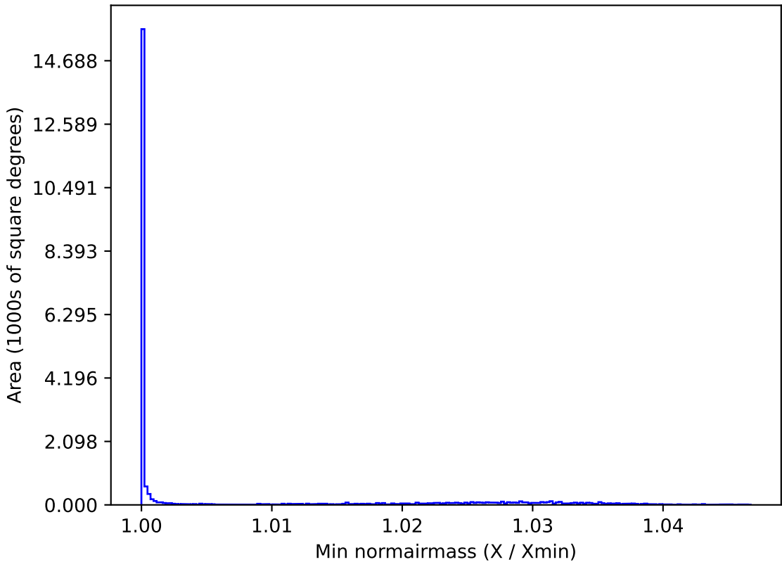
ddf_loaded_fl15_v3.4_10yrs All sky y band: Min normairmass
