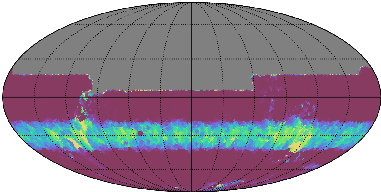
ddf_loaded_fl15_v3.4_10yrs All sky u band: Min normairmass
