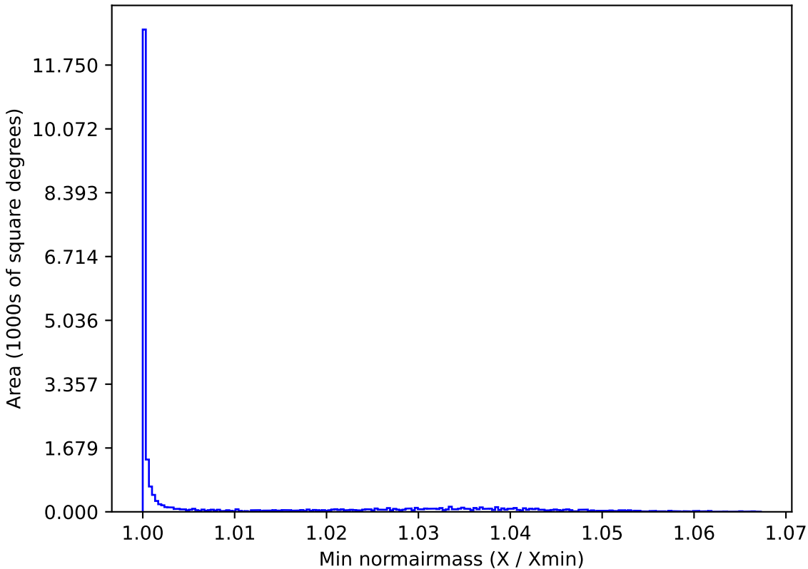
ddf_loaded_fl15_v3.4_10yrs All sky u band: Min normairmass
