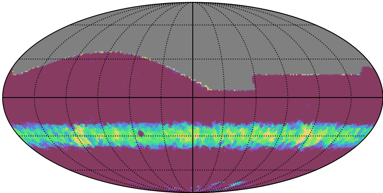
ddf_loaded_fl15_v3.4_10yrs All sky r band: Min normairmass
