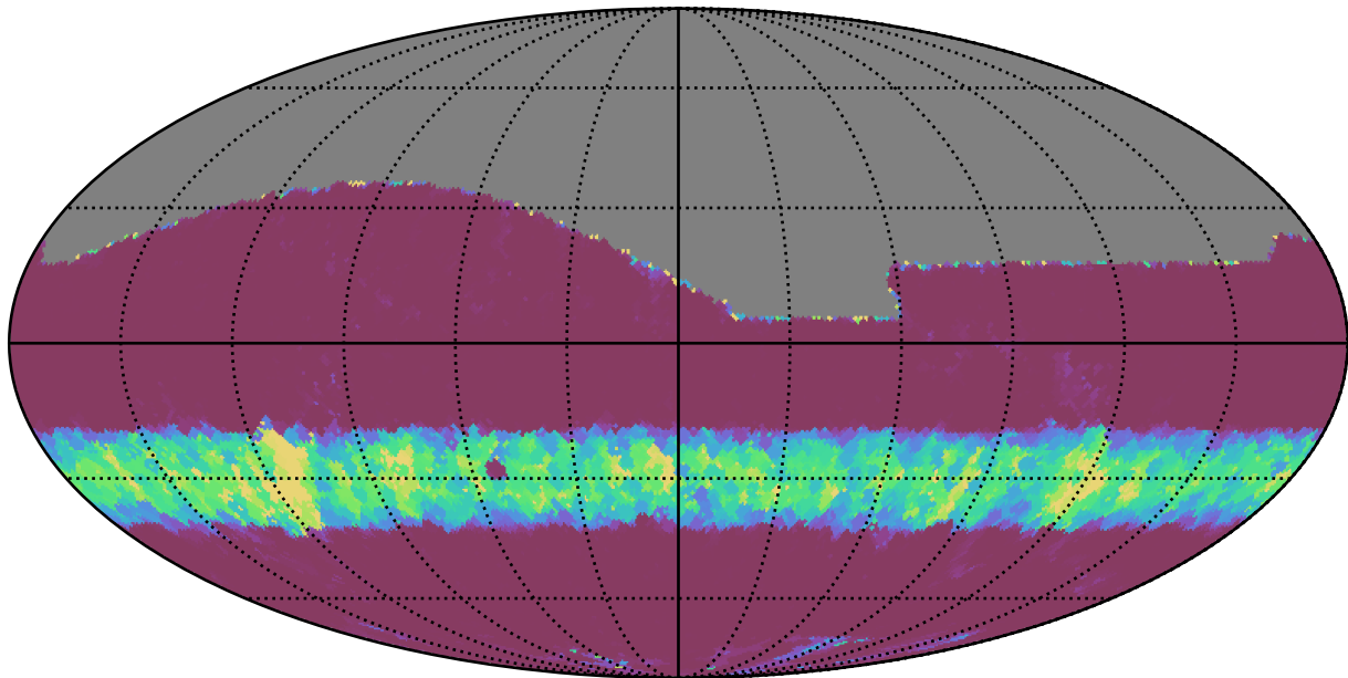
ddf_loaded_fl15_v3.4_10yrs All sky g band: Min normairmass
