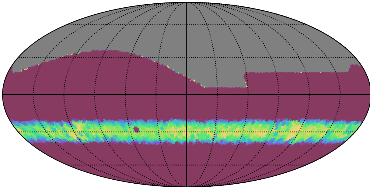
ddf_loaded_fl15_v3.4_10yrs All sky all bands: Min normairmass
