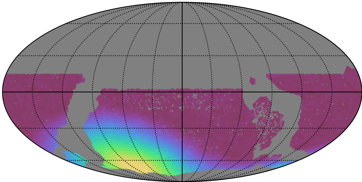
ddf_loaded_fl15_v3.4_10yrs WFD y band: Min moonDistance
