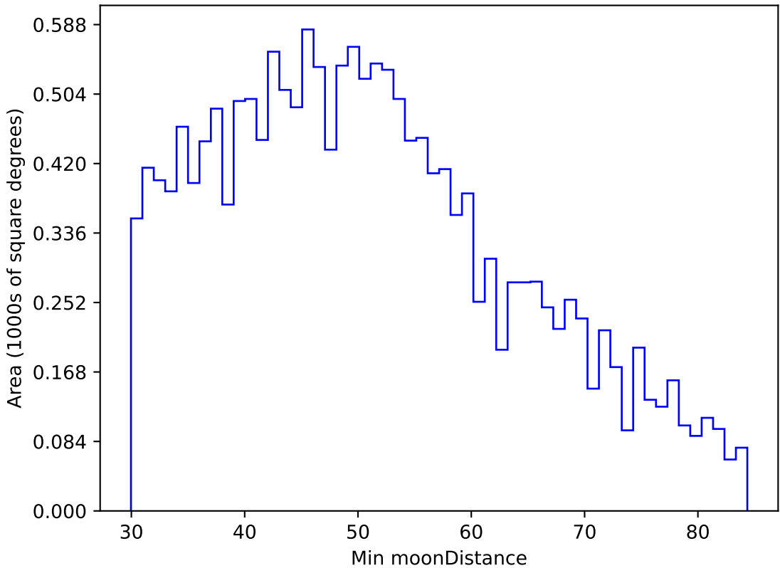
ddf_loaded_fl15_v3.4_10yrs WFD u band: Min moonDistance
