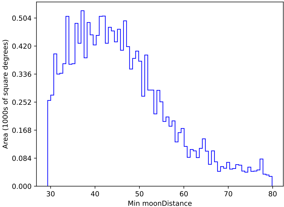
ddf_loaded_fl15_v3.4_10yrs WFD g band: Min moonDistance
