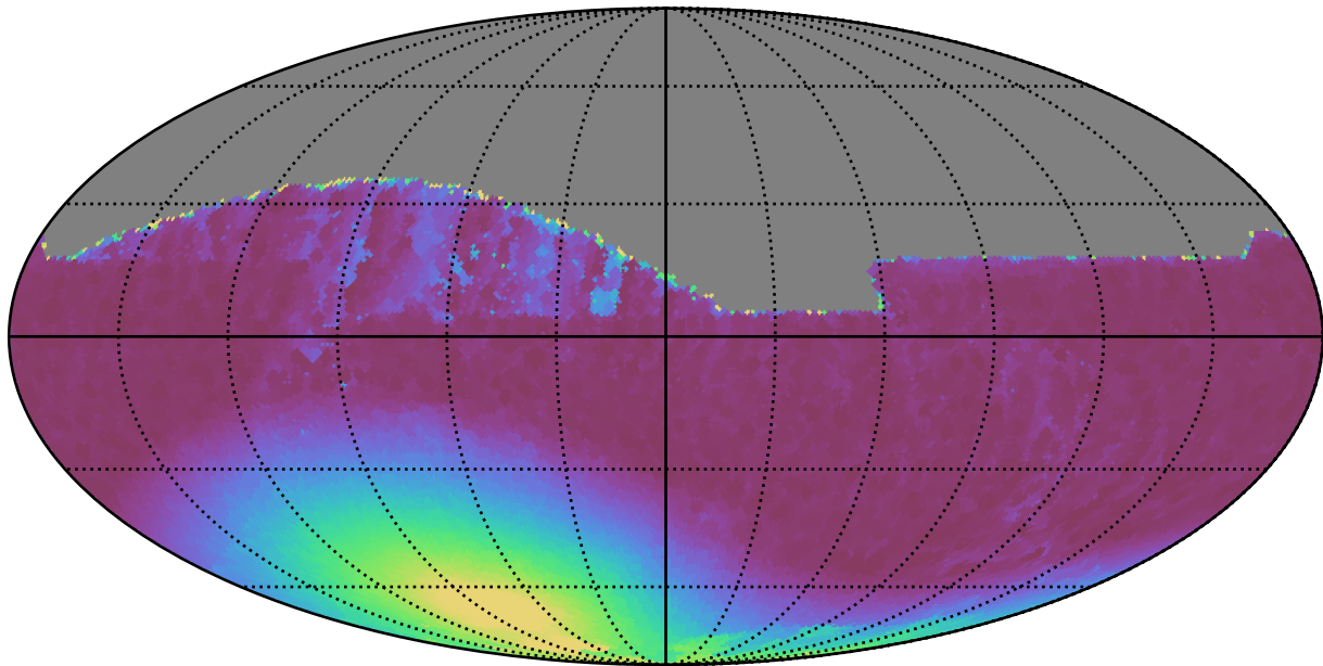
ddf_loaded_fl15_v3.4_10yrs All sky z band: Min moonDistance
