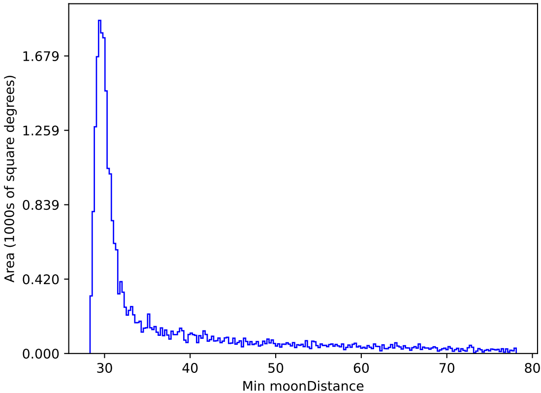
ddf_loaded_fl15_v3.4_10yrs All sky z band: Min moonDistance
