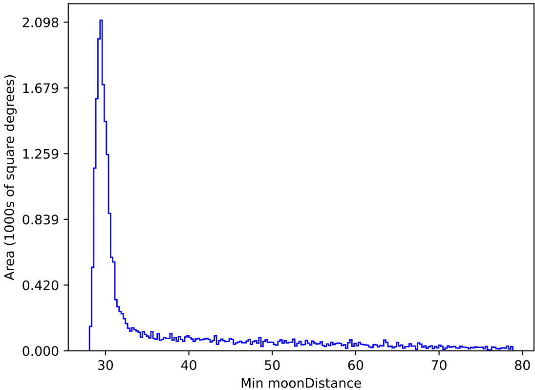
ddf_loaded_fl15_v3.4_10yrs All sky y band: Min moonDistance
