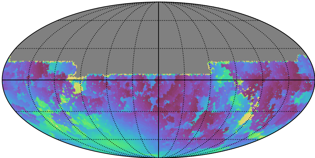
ddf_loaded_fl15_v3.4_10yrs All sky u band: Min moonDistance
