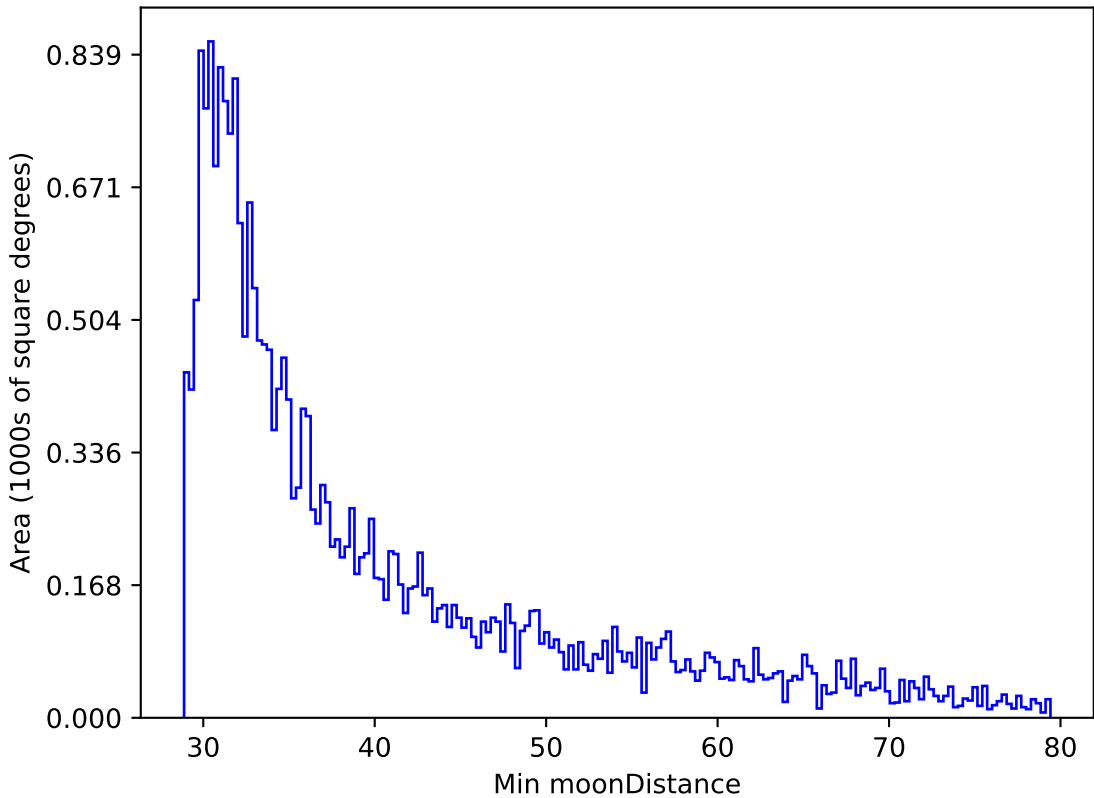
ddf_loaded_fl15_v3.4_10yrs All sky r band: Min moonDistance
