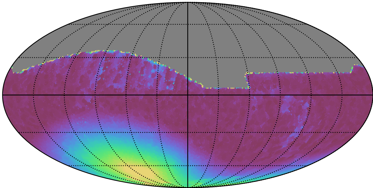
ddf_loaded_fl15_v3.4_10yrs All sky i band: Min moonDistance
