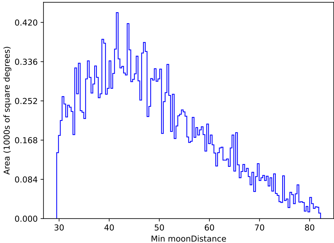
ddf_loaded_fl15_v3.4_10yrs All sky g band: Min moonDistance
