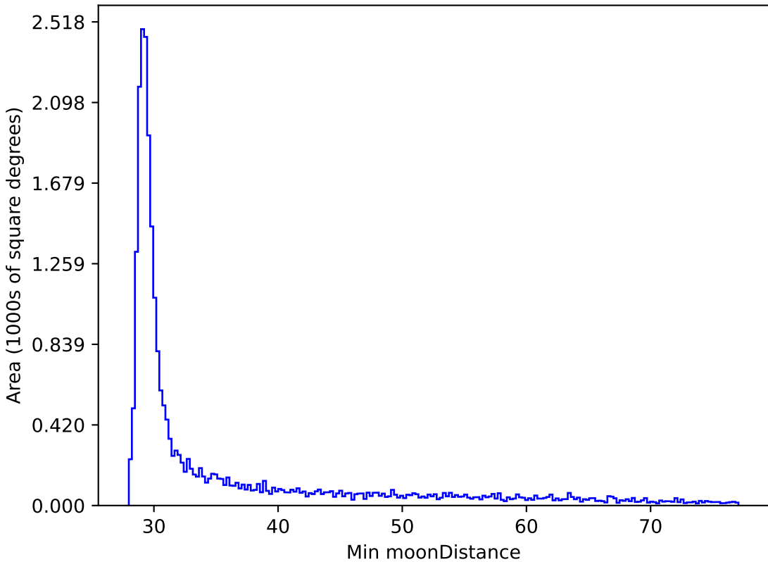
ddf_loaded_fl15_v3.4_10yrs All sky all bands: Min moonDistance
