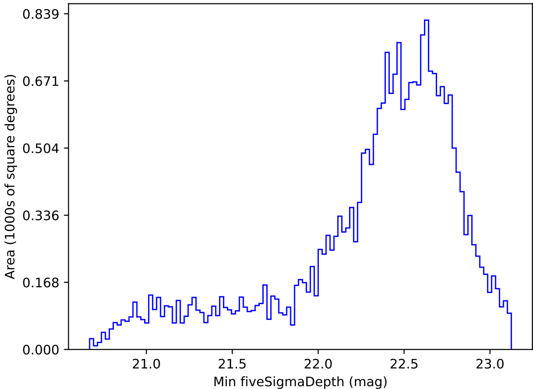
ddf_loaded_fl15_v3.4_10yrs Yr 1 z band: Min fiveSigmaDepth
