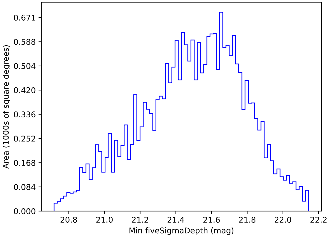
ddf_loaded_fl15_v3.4_10yrs Yr 1 y band: Min fiveSigmaDepth
