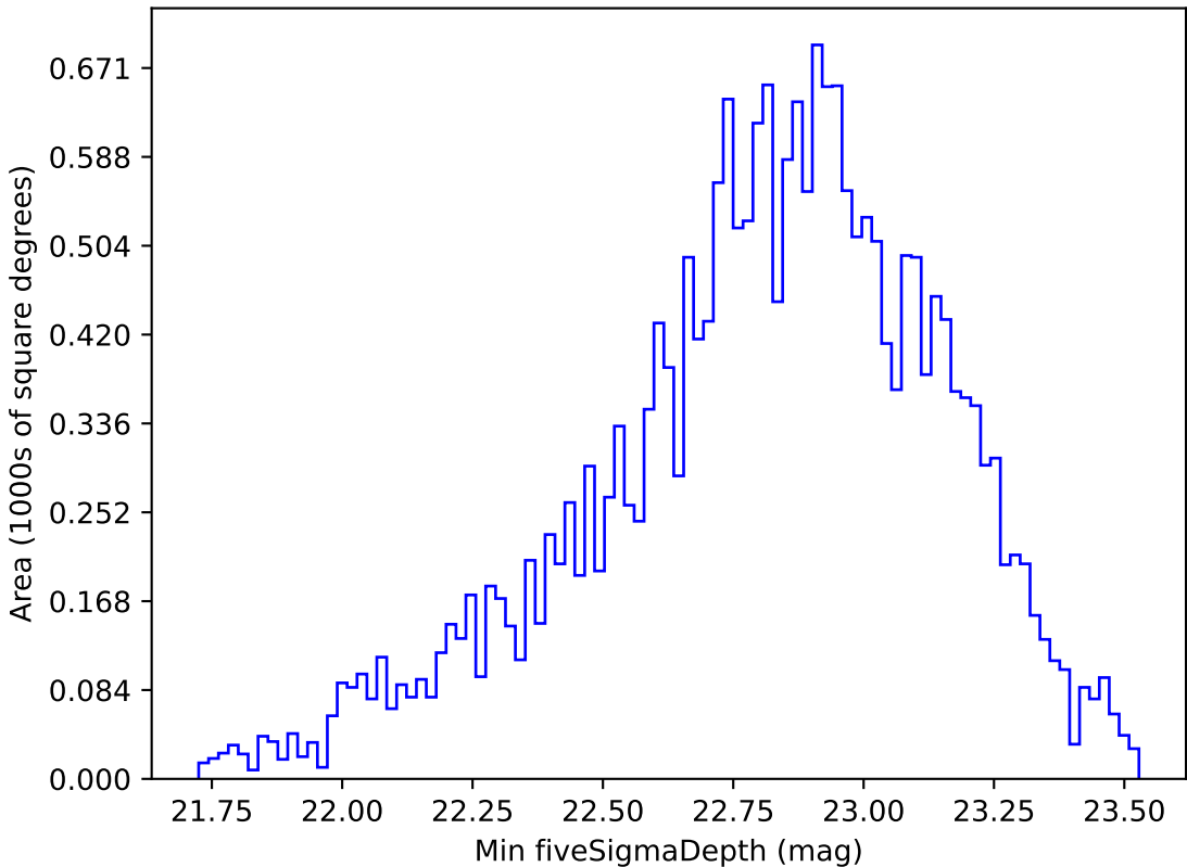
ddf_loaded_fl15_v3.4_10yrs Yr 1 u band: Min fiveSigmaDepth
