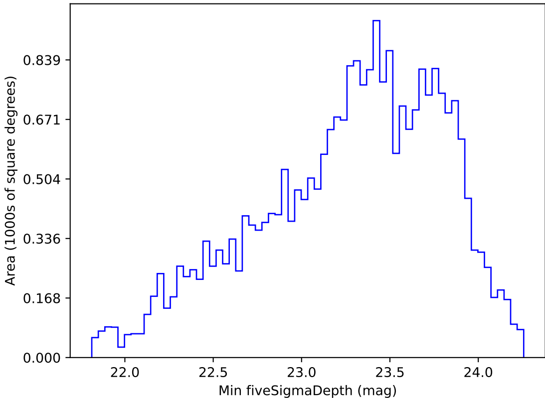
ddf_loaded_fl15_v3.4_10yrs Yr 1 r band: Min fiveSigmaDepth
