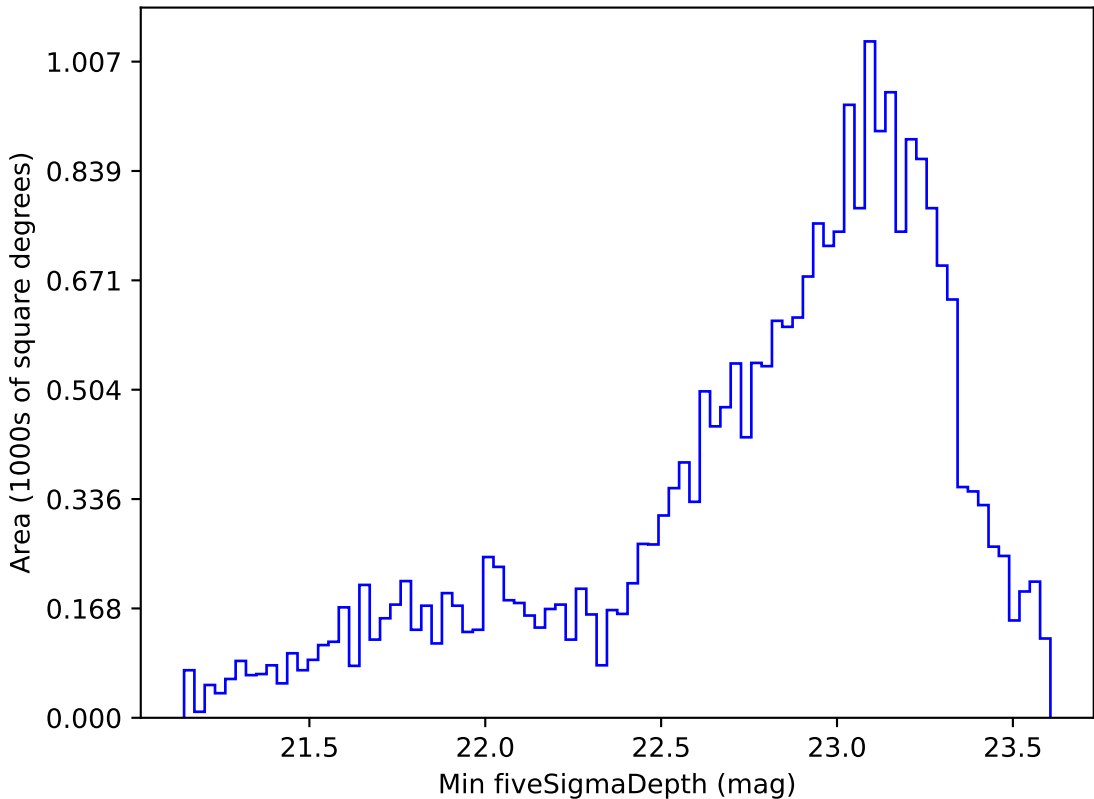
ddf_loaded_fl15_v3.4_10yrs Yr 1 i band: Min fiveSigmaDepth
