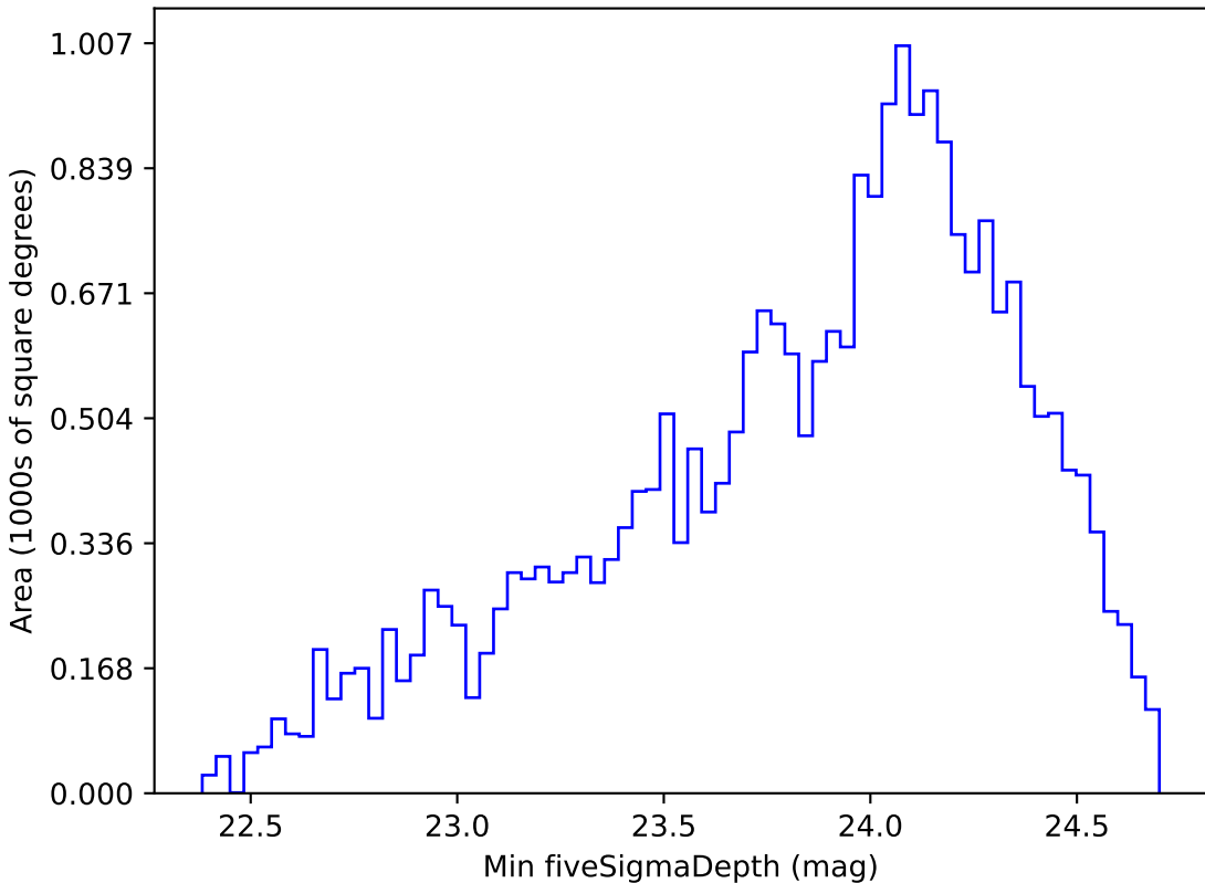
ddf_loaded_fl15_v3.4_10yrs Yr 1 g band: Min fiveSigmaDepth
