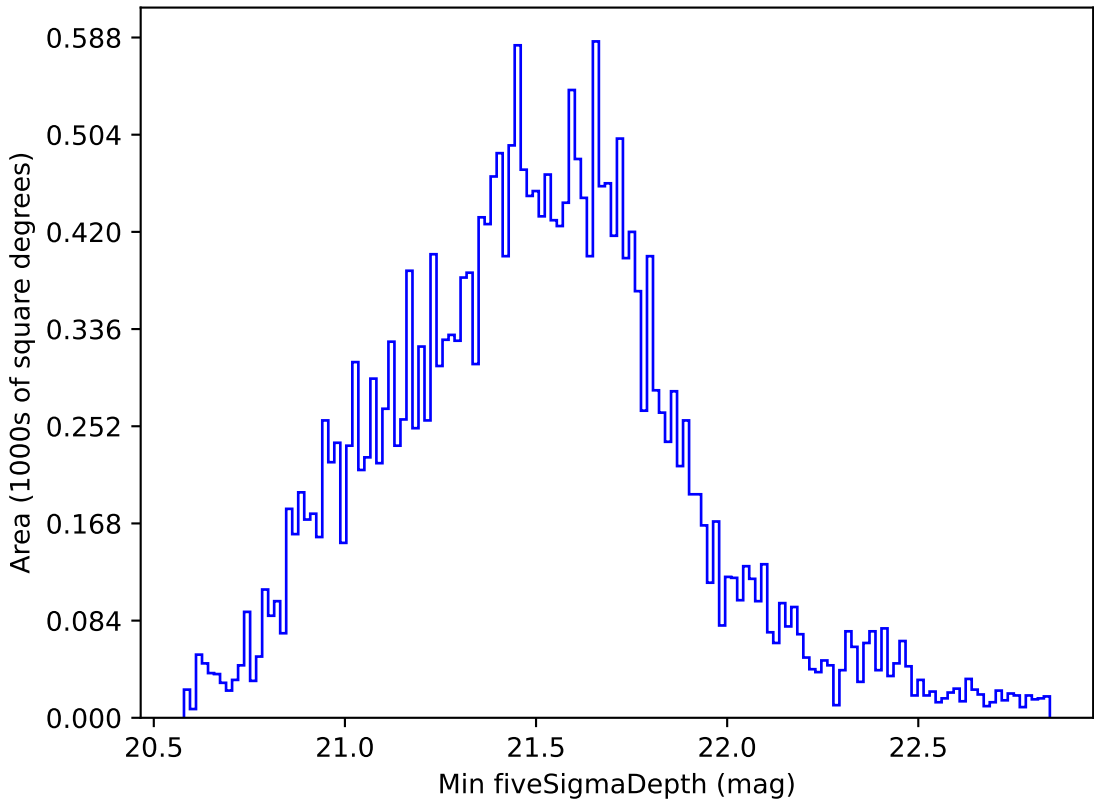
ddf_loaded_fl15_v3.4_10yrs Yr 1 all bands: Min fiveSigmaDepth
