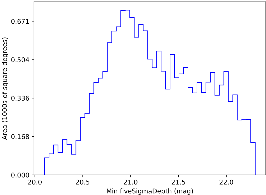
ddf_loaded_fl15_v3.4_10yrs WFD z band: Min fiveSigmaDepth
