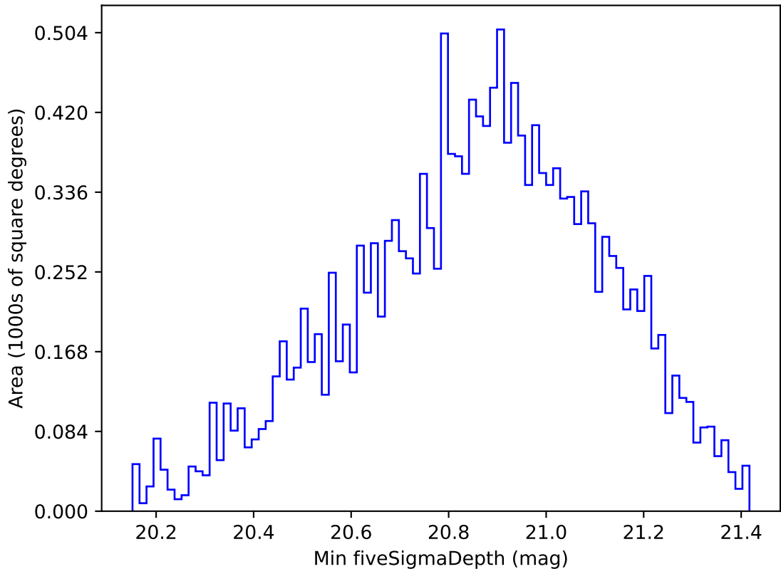
ddf_loaded_fl15_v3.4_10yrs WFD y band: Min fiveSigmaDepth
