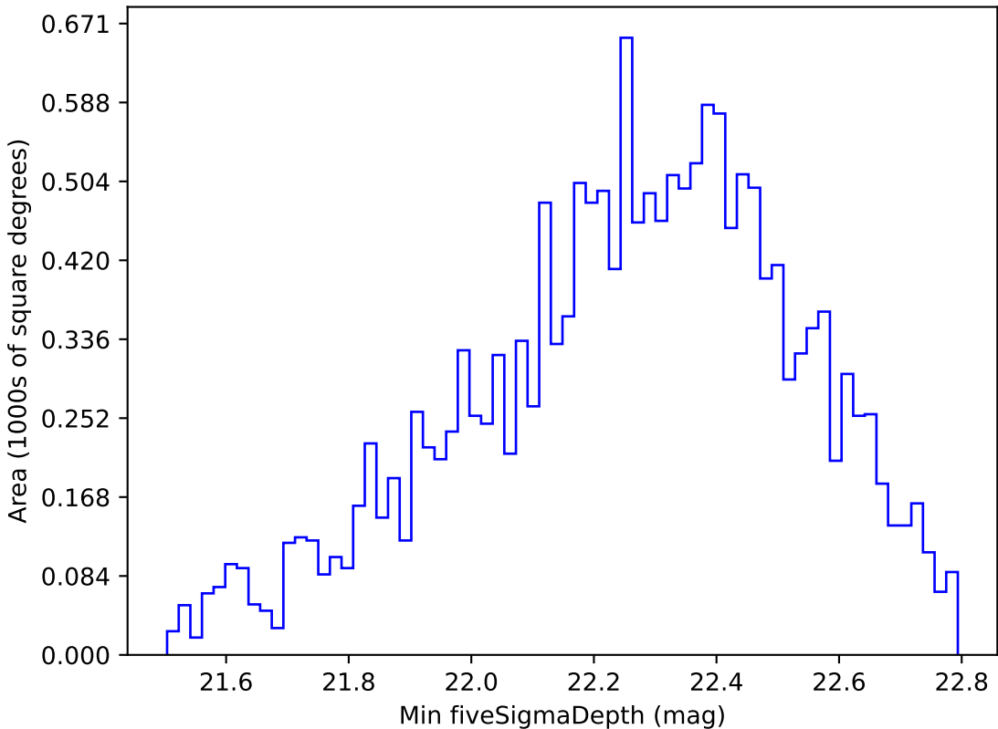
ddf_loaded_fl15_v3.4_10yrs WFD u band: Min fiveSigmaDepth
