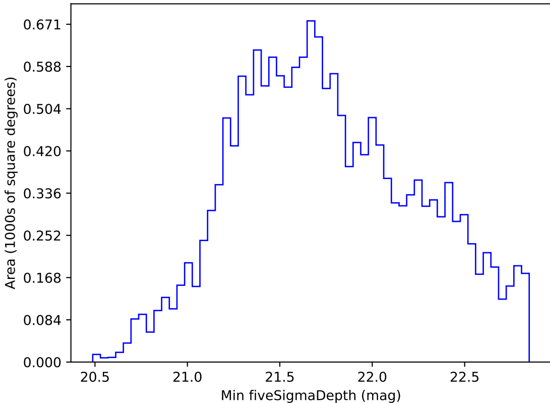
ddf_loaded_fl15_v3.4_10yrs WFD i band: Min fiveSigmaDepth
